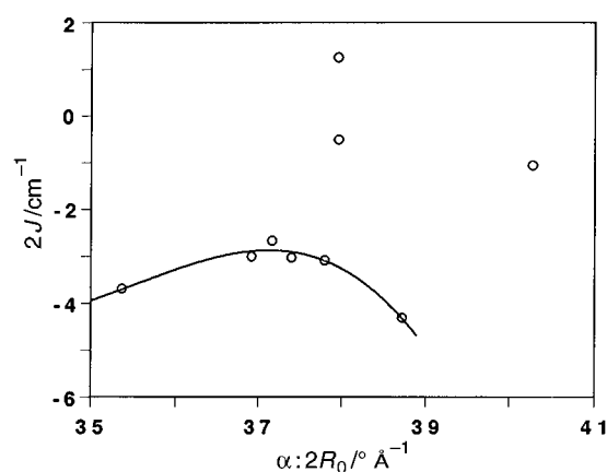
Fig. 7 Variation of 2J vs. \alpha:2R_0
