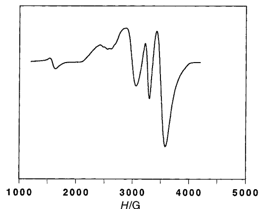
Fig. 4 The EPR powder spectrum (X-band) of [Cu(tzq) 2 (HCO 2 ) 2 ](μ-HCO 2 ) 2 ·4H 2 O at 4.2 K
