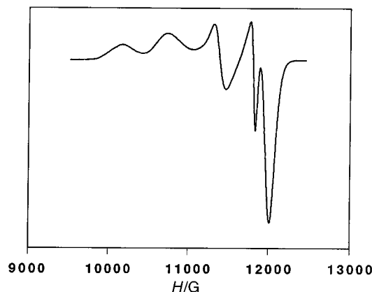
Fig. 3 The EPR powder spectrum (Q-band) of [Cu(tzq) 2 (HCO 2 ) 2 ](μ-HCO 2 ) 2 ·4H 2 O at room temperature
